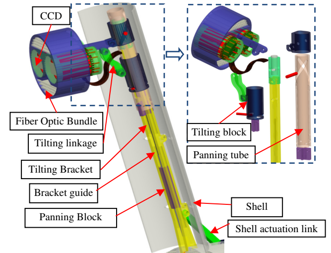
Fig. 2. Camera module of the IREP
