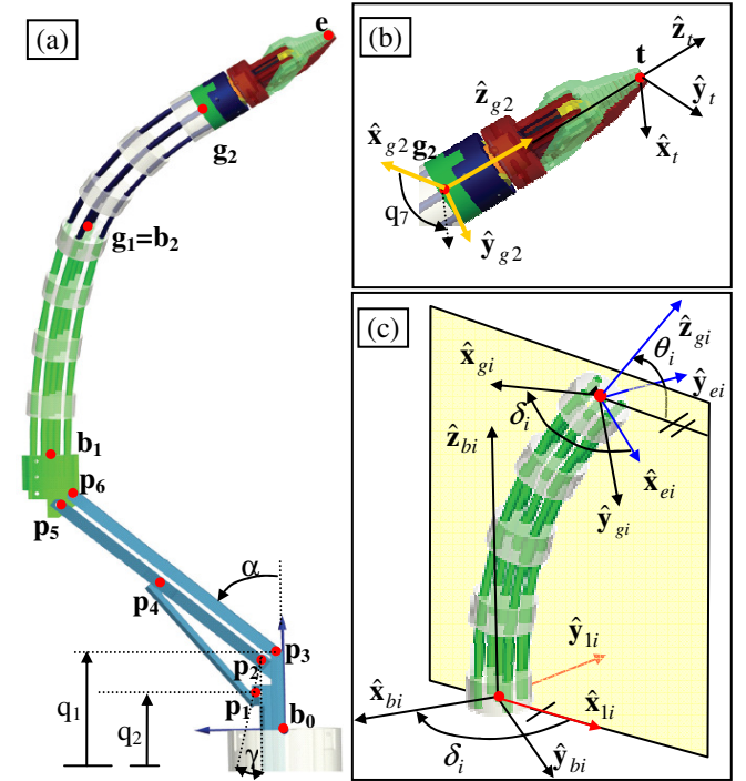
Fig. 4. Nomenclature of a single dexterous arm of the IREP: (a) definition of points, (b) definition of the tip frame and the wrist rotation angle q_7 , (c) definition of local frames for the i^{th} segment of the continuum robot
